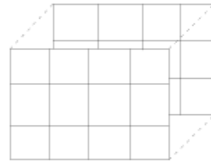
Result: 3-by-4-by-2
