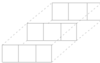
B: 1-by-3-by-3
