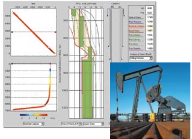
One of GMI’s graphical user interfaces, used by drilling engineers at the wellhead to determine optimum mud weights.
