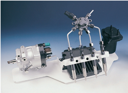
Delphi Diesel common rail system.
