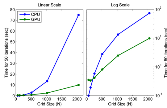
Figure 4. Linear scale plot (left) and log scale plot (right) of the same benchmarks results showing the time required to complete 50 time steps at different grid sizes.
