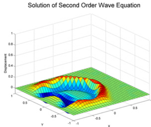
Figure 2. A solution for a second-order wave equation on a 32 x 32 grid.
