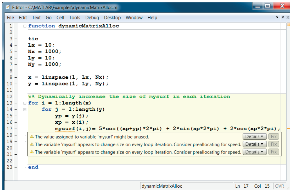
Figure 5. Sample MATLAB Code Analyzer results.
